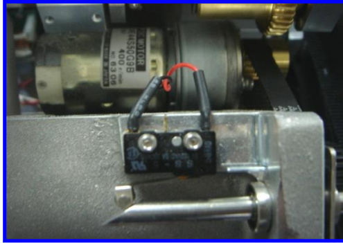
<HARNESS(CLAMP LIMIT SWITCH(M.J12))>
