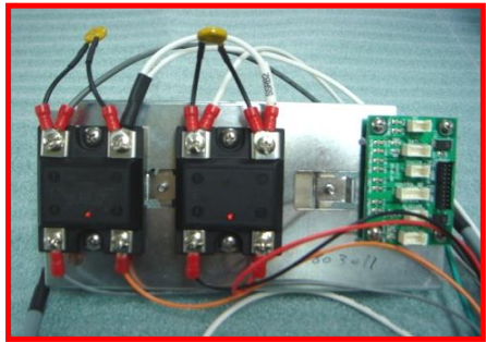
<B-1. ELECTRIC SSR ASS'Y>
