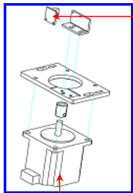
<B-1. ELECTRIC SSR ASS'Y>
